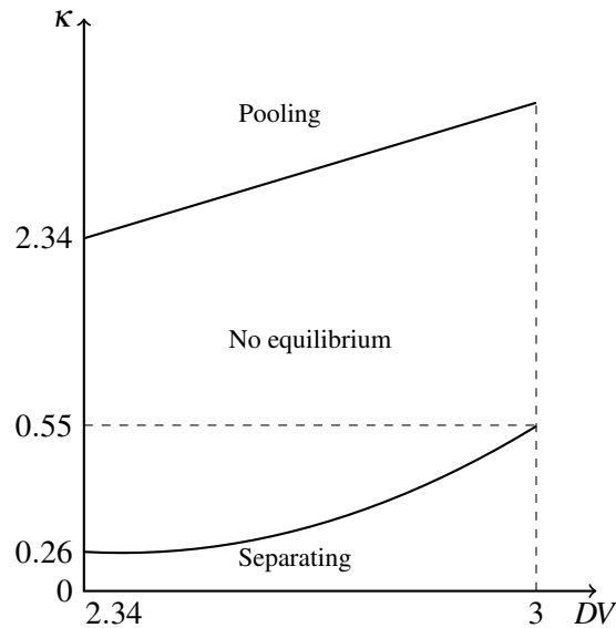
Figure 1: Equilibria when t = 1 , q = 0.85 and DV \in [2.34, 3] .
